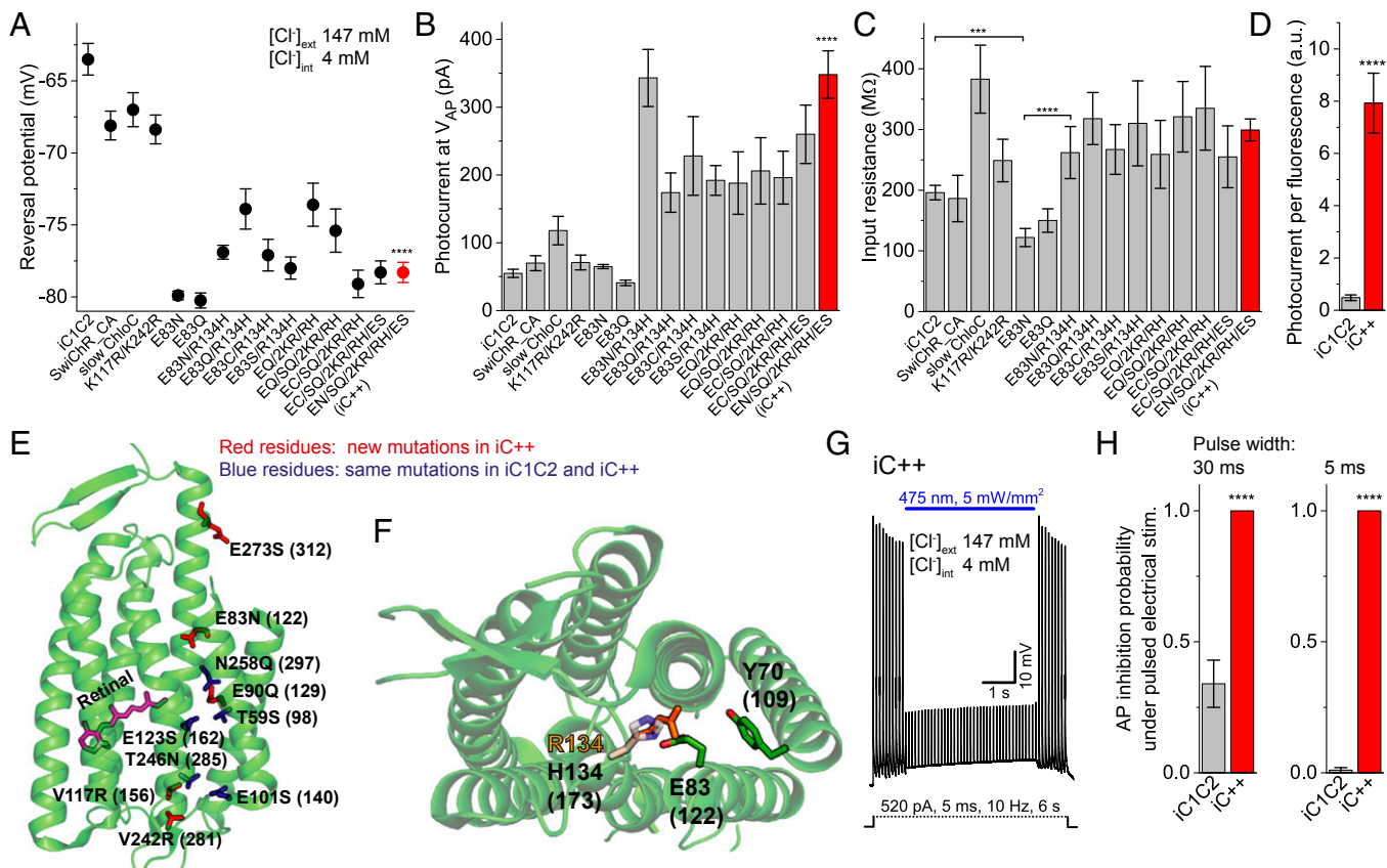
Fig. 1. Design and characterization of iC++ in cultured neurons of rat hippocampus. ( A ) V_{rev} of iC1C2 mutations compared with chloride-conducting channelrhodopsins at an intracellular chloride concentration of 4 mM. EN/Q/C: E83N/Q/C; ES: E273S; RH: R134H; SQ: S90Q; 2KR: K117R/K242R. ( B ) Photocurrent amplitudes measured at the V_{AP} ( -51 \pm 4 mV). ( C ) R_{in} of channelrhodopsin-expressing cells. ( D ) Stationary photocurrents per fluorescence of eYFP-tagged constructs expressed in cultured neurons. ( E ) C1C2 structure depicting iC++ mutations. Numbering refers to N-terminal-truncated channel iC++. Corresponding positions in the original C1C2 structure are indicated in parentheses. ( F ) Structural model of the putative cytosolic ion gate in C1C2. Histidine 134 (173) (gray) was replaced by arginine in iC1C2 (orange) but not in iC++. ( G ) Voltage trace of a cultured neuron expressing iC++. APs were evoked by pulsed electrical inputs at 10 Hz (dotted line) and were inhibited by continuous light application (blue bar) for 4 s. ( H ) Inhibition probability of APs evoked by pulsed current injections (6 s, 10 Hz) with pulse widths of 30 ms (Left), and 5 ms (Right) under 4-s light application. Current inputs were individually titrated to the V_{AP} . Shorter pulses required stronger current amplitudes. Average: 30 ms: 202 \pm 11 pA; 5 ms: 559 \pm 40 pA. pH_{ext} = 7.3 , pH_{int} = 7.2 ; [Cl^-]_{ext} = 147 mM, [Cl^-]_{int} = 4 mM for entire figure. ***P < 0.005 , ****P < 0.0001 . Error bars indicate SEM; all values and numbers are listed in SI Appendix , Table S1.
